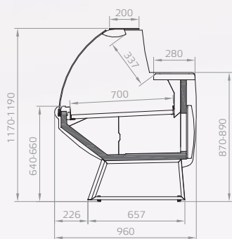
newKRISTINA V
