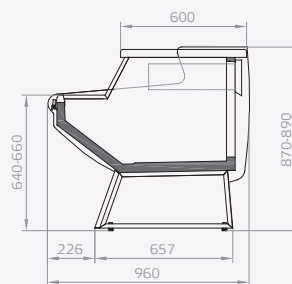
newKRISTINA MP
